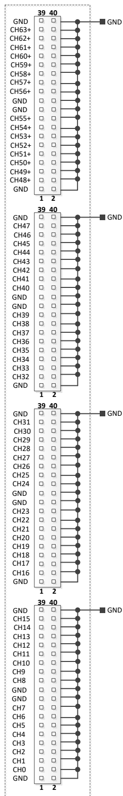
2mm 40-pin headers female
