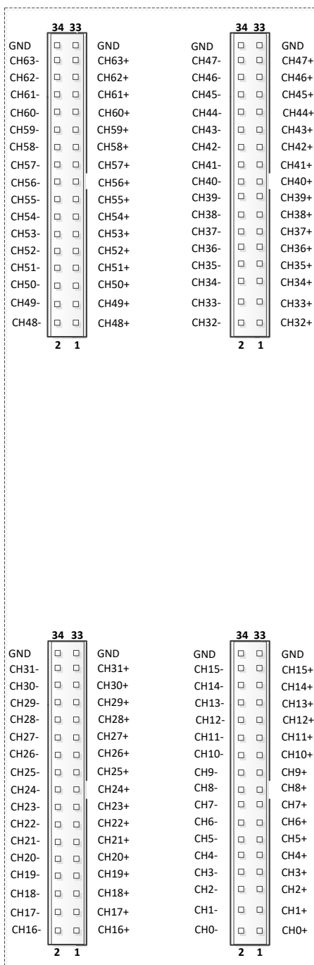
Front View
