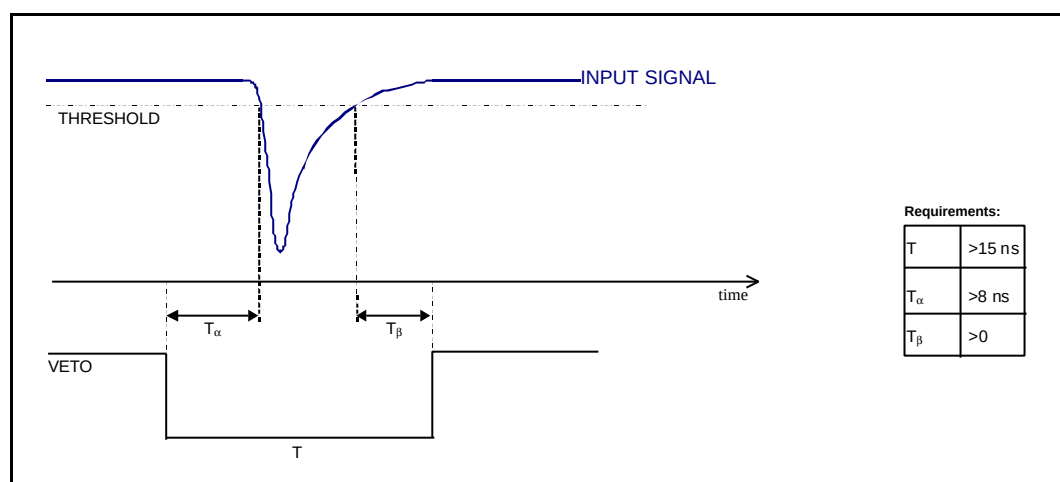
Fig. 2.1: Veto signal
