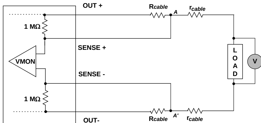
Fig. 3.3 – LDR system + remote voltage sensing scheme
