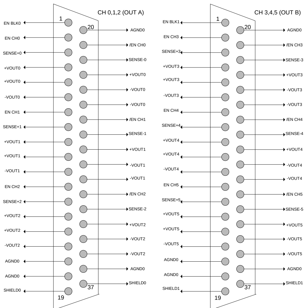
Fig. 3.1 - Mod. A 1518 B Pin assignment
