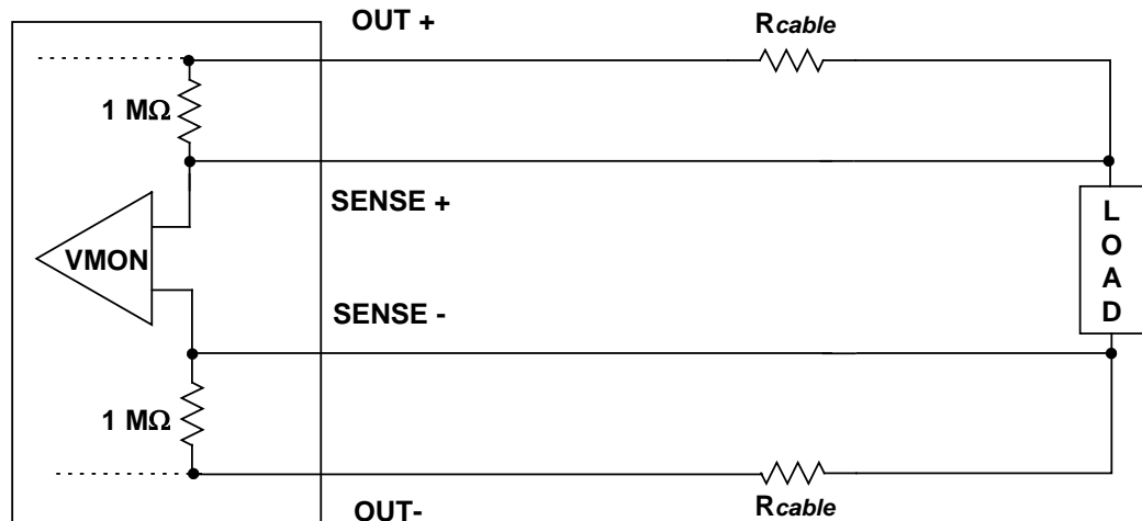
Fig. 3.2 - Remote voltage sensing scheme
