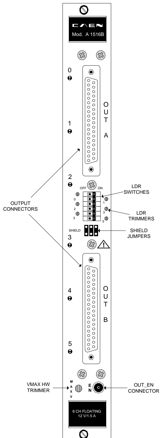
Fig. 1.1 - Mod. A 1516 B front panel
