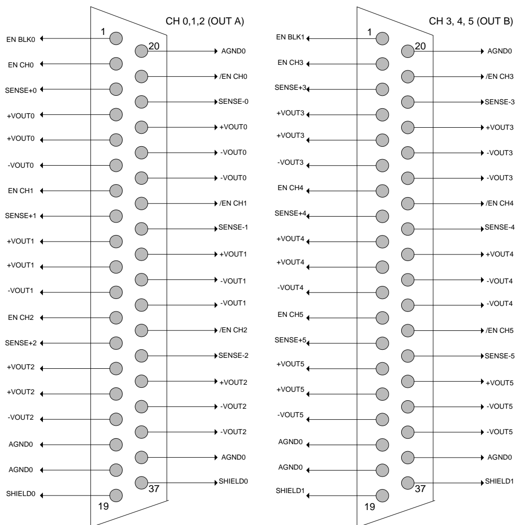
Fig. 3.1 - Mod. A 1516 B Pin assignment
