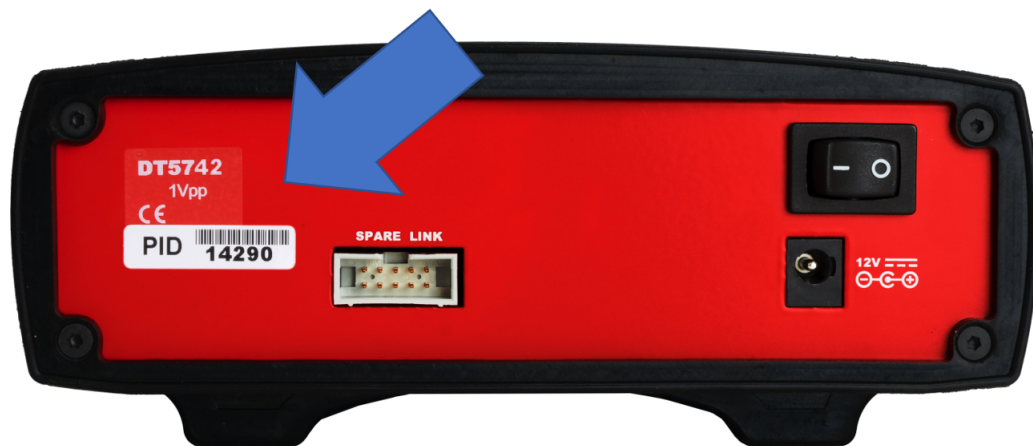
Fig. 5.1: PID location on DT5742 (the number in the picture is purely indicative)
