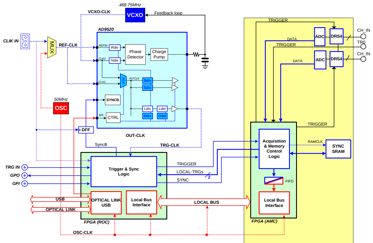
Fig. 9.4: Clock distribution diagram
