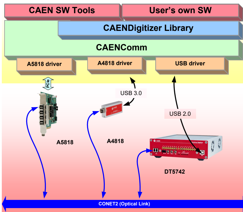
Fig. 10.1: Drivers and software layers
