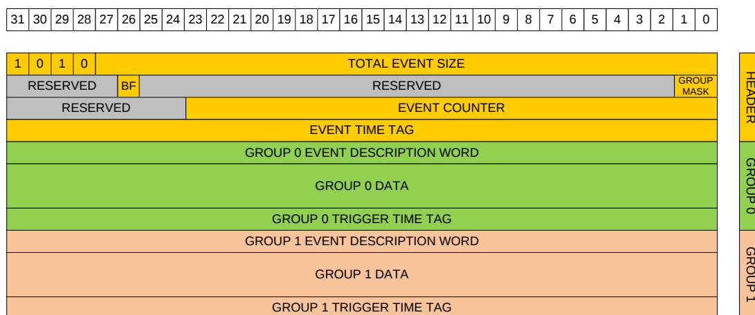
Fig. 9.12: Event Format
