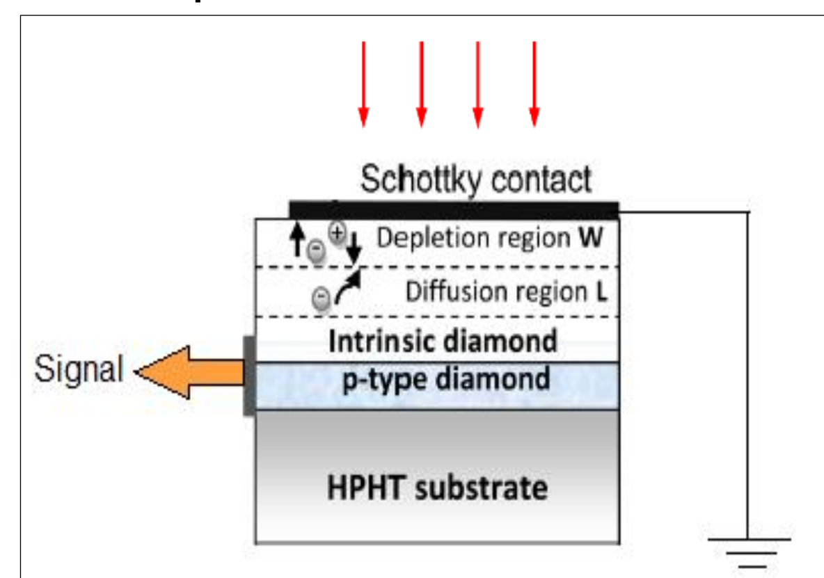
Figure 2: Structure of the diamond photodetector in layered layout (top), and some events detected by diamonds on FTU (bottom). In this case, diamond signals are compared to machine diagnostics: MHD activity (bottom left) and MARFE (bottom right) are clearly recognizable [3].
