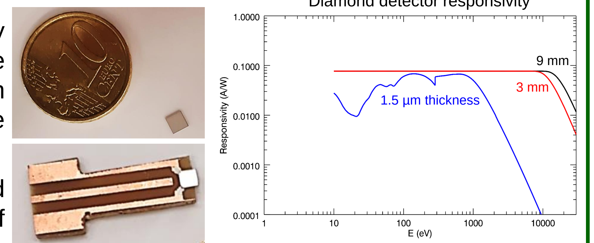
Figure 1: Pictures of a CVD diamond layer and example of detector layout (left), and calculation of the approximated detector's responsivity to photons of different energies for various diamond active layer thicknesses (right) [2].
