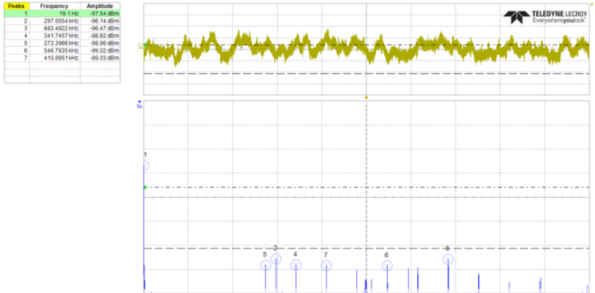
Output frequency spectrum. 500ms integration time
