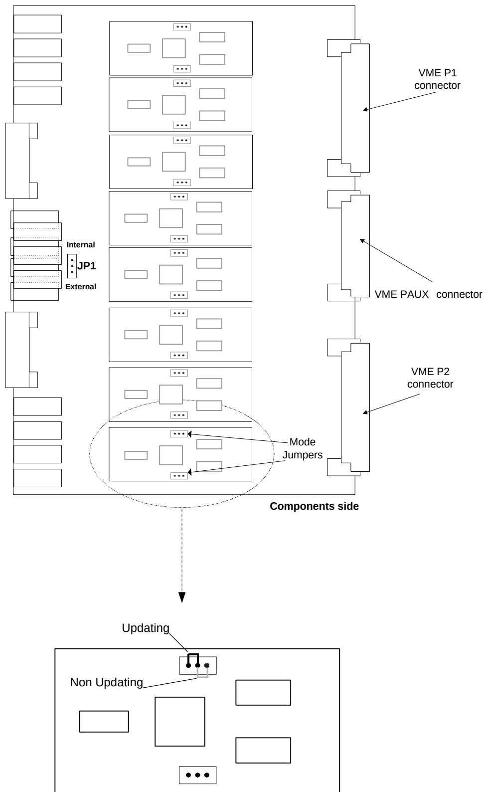
Fig. 2.3: Jumpers location
