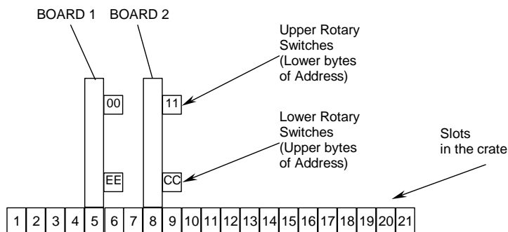
Fig. 4.5: Base/GEO Addressing: Example 1
