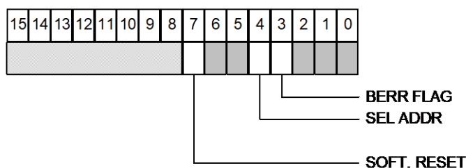
Fig. 4.15: Bit Set 1 Register
