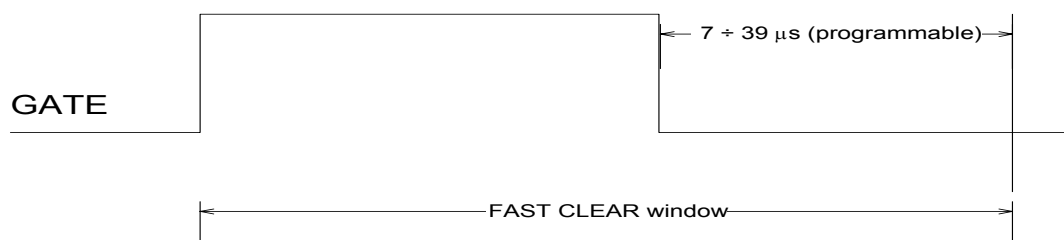
Fig. 2.9: Fast Clear window
