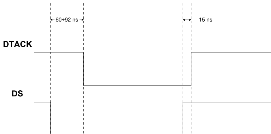
Fig.A.2: VME cycle timing in BLT/CBLT mode
