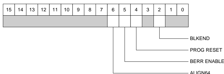
Fig. 4.17: Control Register 1
