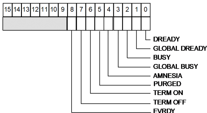
Fig. 4.16: Status Register 1
