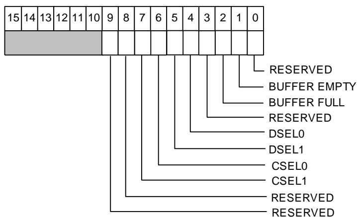
Fig. 4.22: Status Register 2
