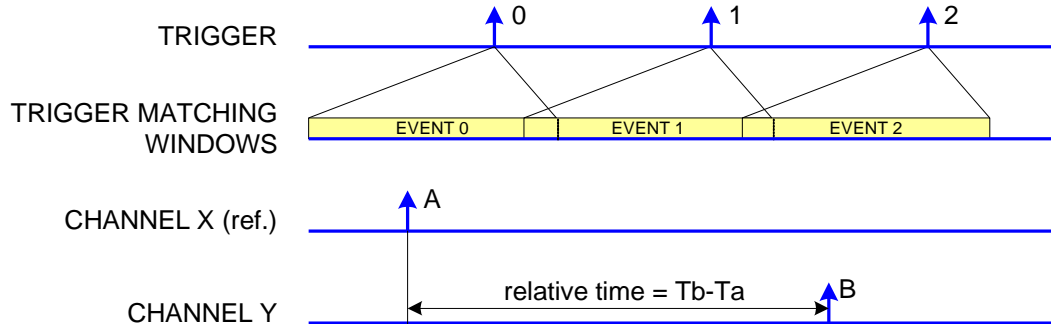
Fig. 2.9: Using the trigger in the long scale time measurements
