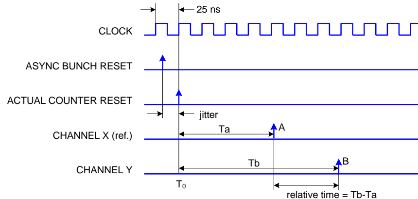
Fig. 2.8: Relative Time measurement
