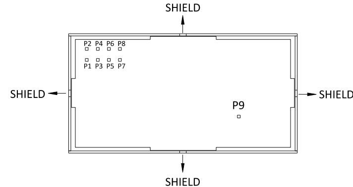
Fig. 4: A7526 pins position (bottom view)
