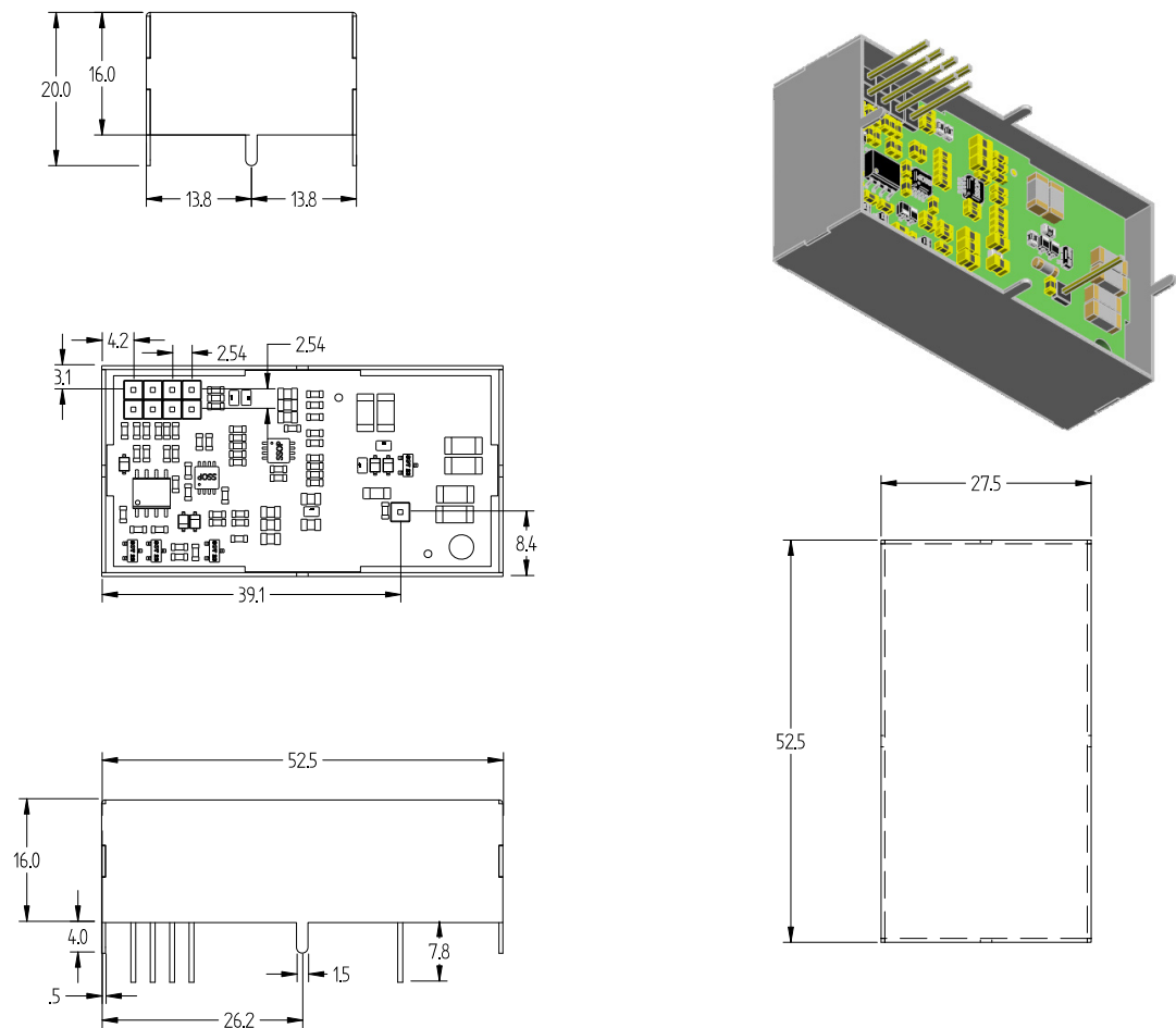
Fig. 3: A7526 External packaging (all dimension in mm)
