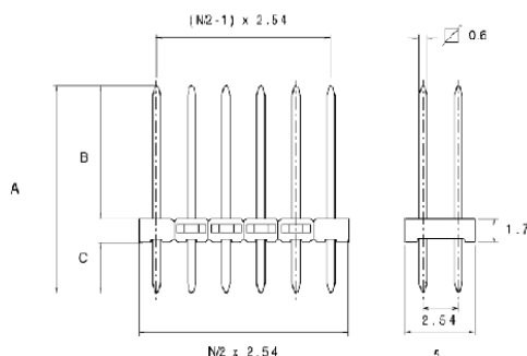
Fig. 2: Male strip header of A7526
