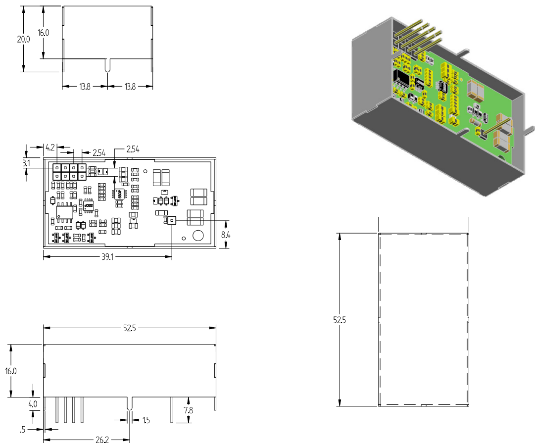
Fig. 3: A7520 External packaging (all dimension in mm)
