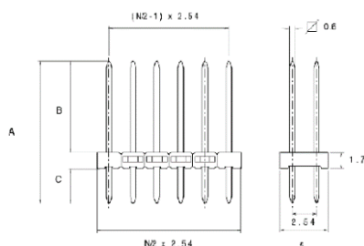
Fig. 2: Male strip header of A7520
