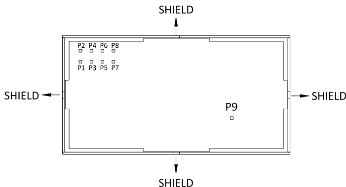
Fig. 4: A7520 pins position (bottom view)
