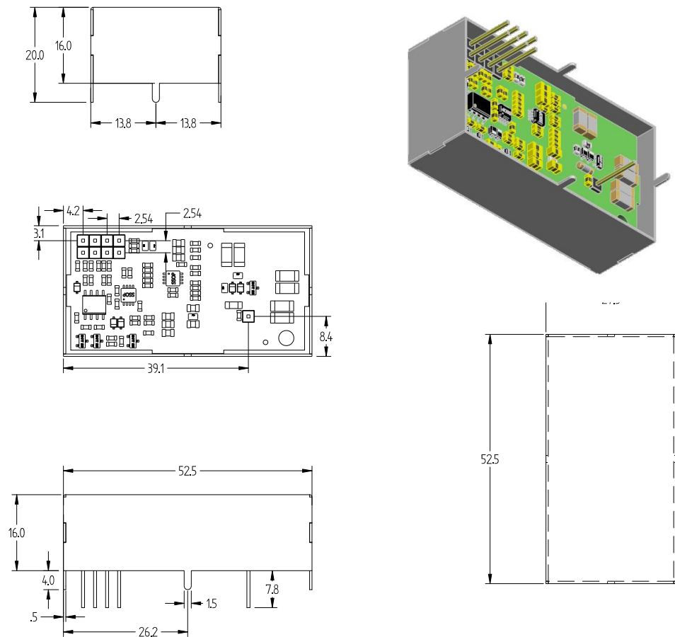
Fig.5: A7504C External packaging (all dimensions in mm)
