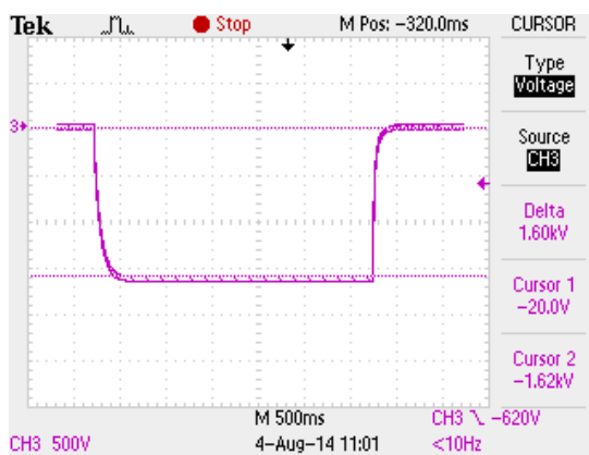
Fig.3: Vout at turning On and Off (Load = 2.6 M \Omega )
