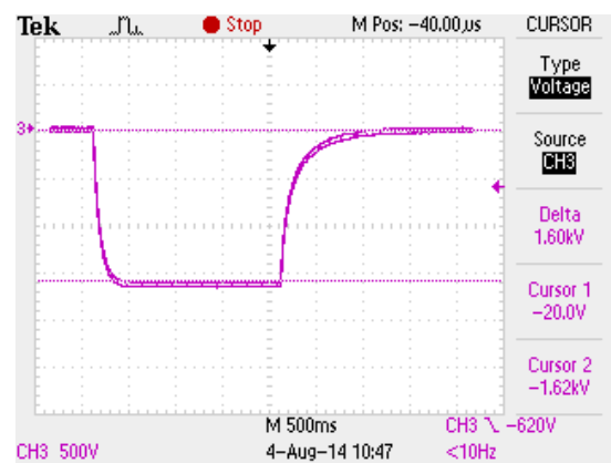
Fig.4: Vout at turning On and Off (Load = 20 M \Omega )
