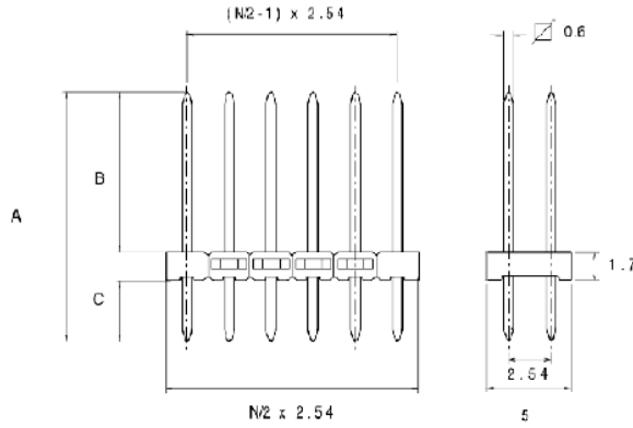
Fig.2: Male strip header of A7504C
