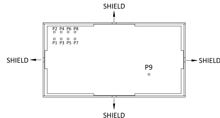
Fig.6: A7504C pins position (bottom view)
