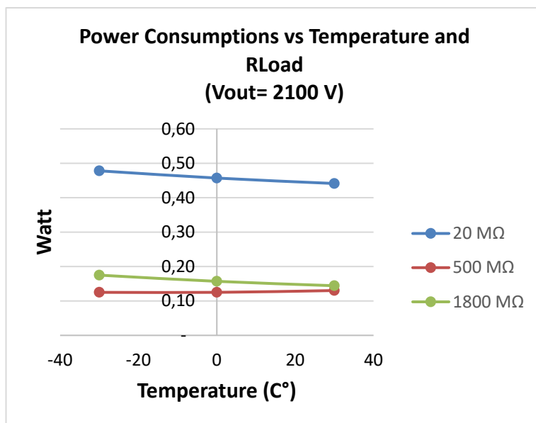
Fig. 4: Power consumptions @ 2100 V vs Temperature
