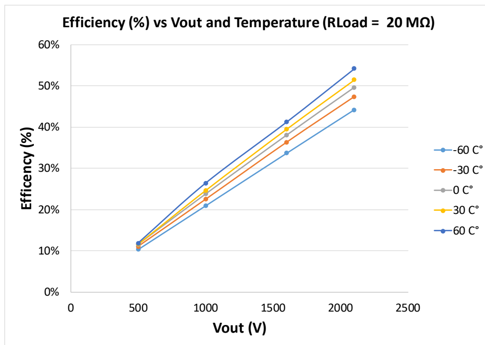
Fig. 3: Efficiency vs Vout and Temperature
