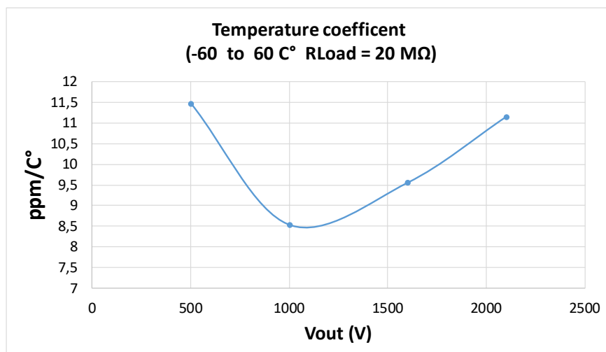
Fig. 5: Temperature coefficient vs Vout
