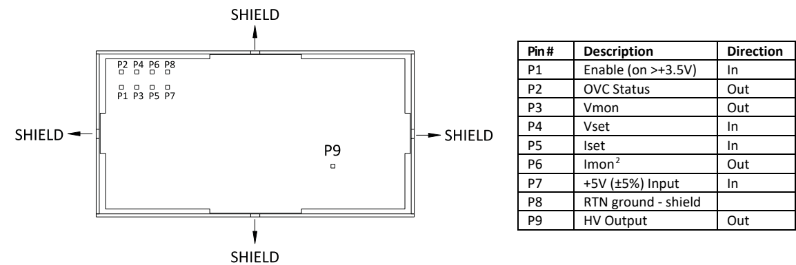
Fig. 10: A7502 pins position (bottom view)
