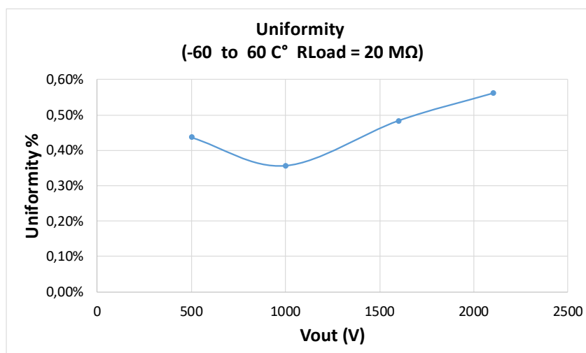
Fig. 6: Uniformity of a Lot ( \Delta V_{out}/V_{out} )
