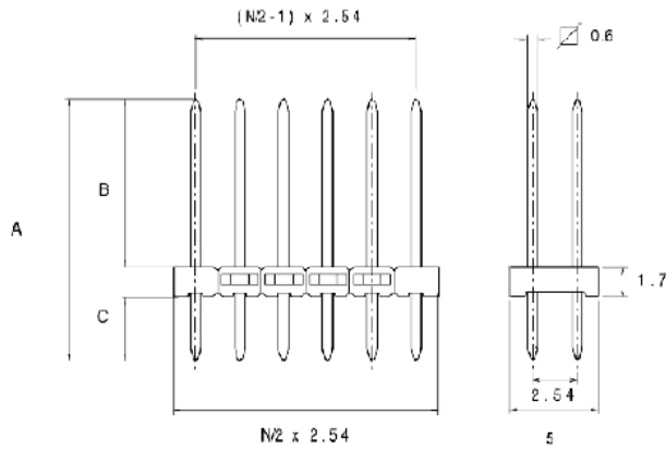
Fig. 2: Male strip header of A7502
