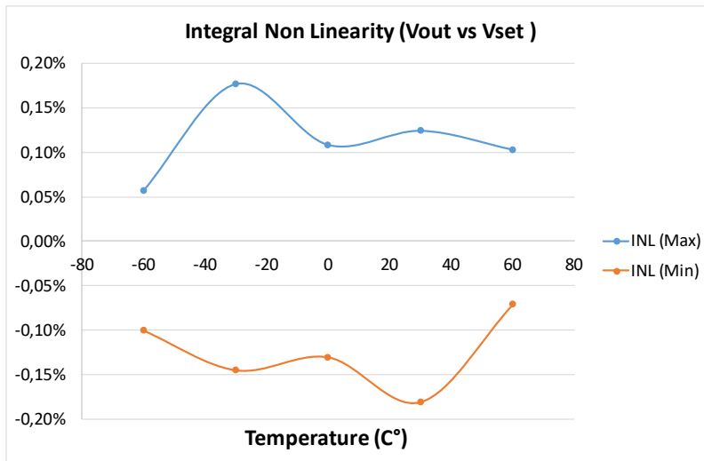
Fig. 7: Integral non-linearity ( \Delta V_{out}/V_{out} )
