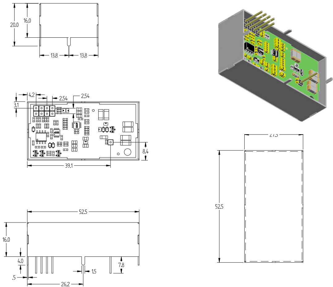
Fig. 9: A7502 External packaging
