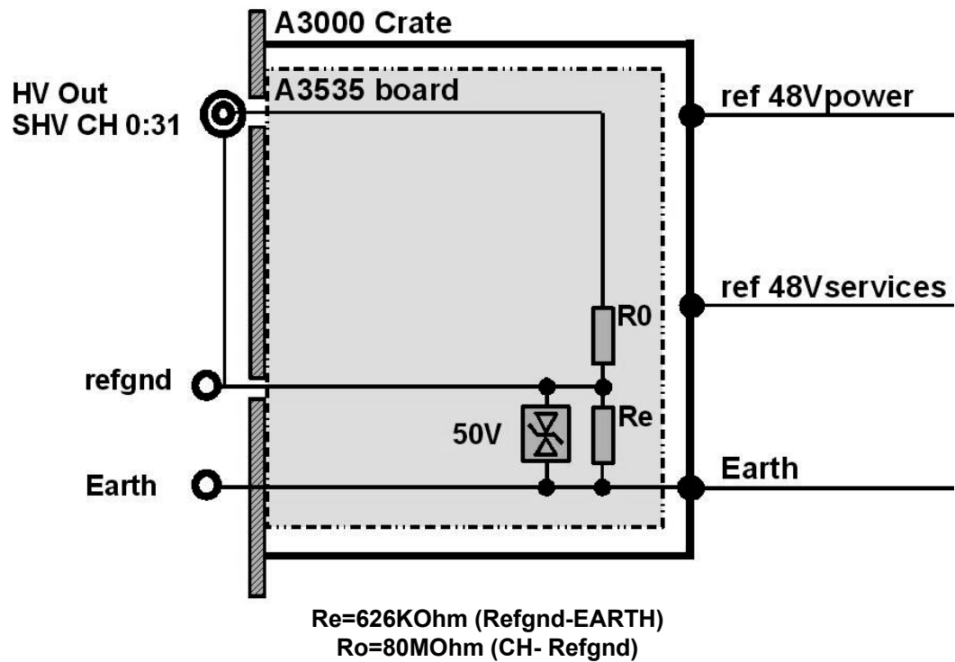
Fig. 2.2 – A3535 Channels ground scheme
