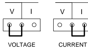
Fig. 4.3 – VMAX / IMAX jumpers setting
