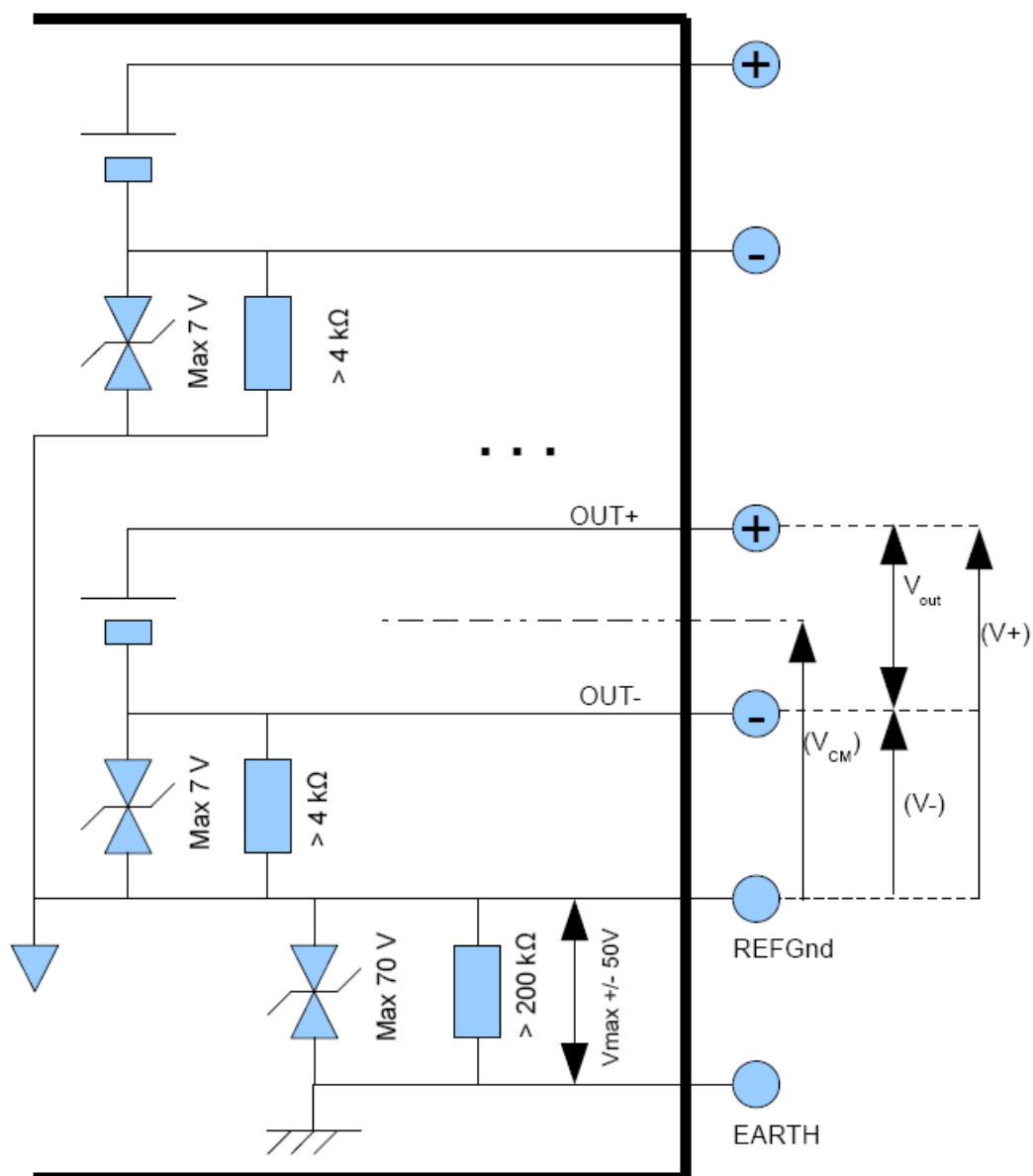
Fig. 2.3 – A3016 Channels ground scheme
