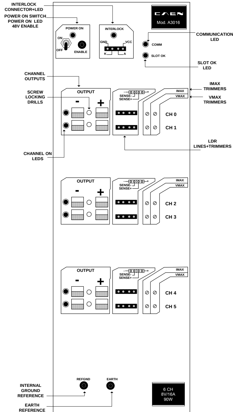
Fig. 2.1 – A3016 Front Panel
