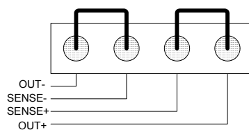
Fig. 4.3 – SENSE connector
