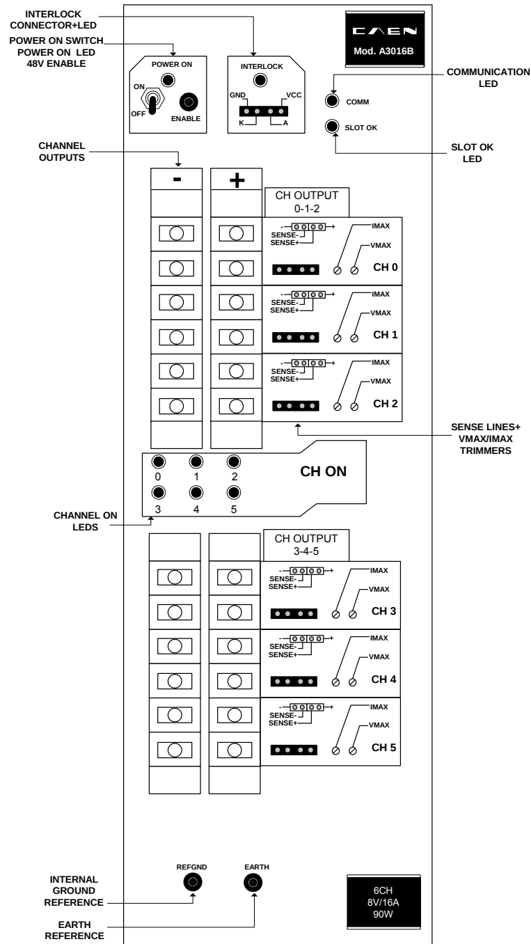
Fig. 2.2 – A3016B Front Panel
