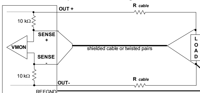
Fig. 5 – Remote voltage sensing scheme
