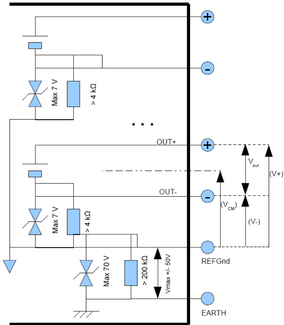
Fig. 2 – Ground scheme
