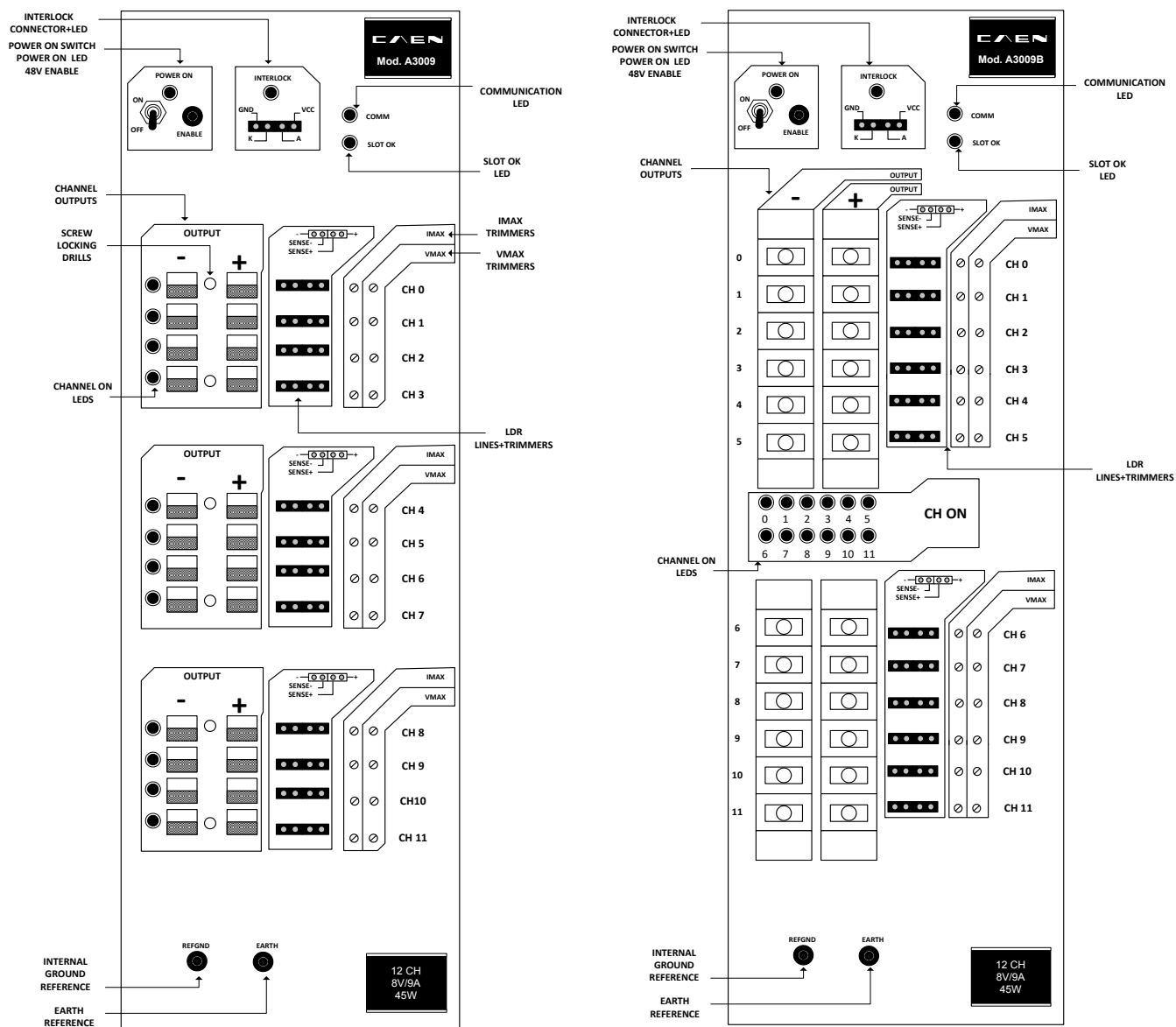
Fig. 1 – A3009 and A3009B front panel
