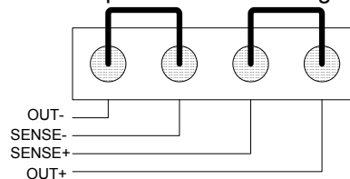
Fig. 4.3 – SENSE connector
