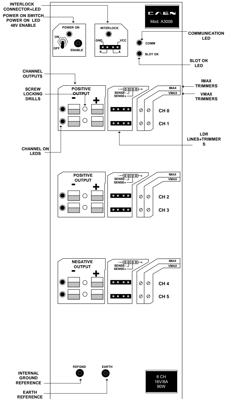
Fig. 2.1 – A3006 Front Panel
