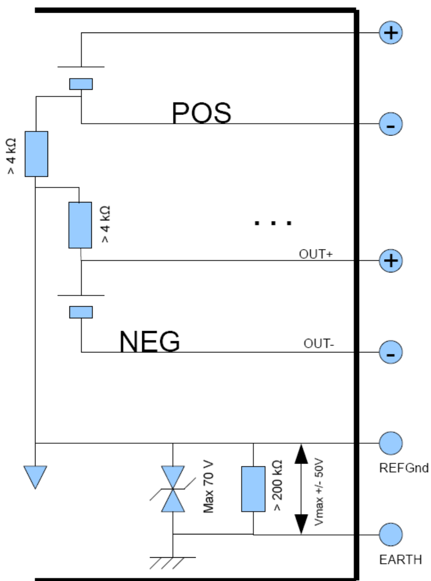
Fig. 2.2 – A3006 Channels ground scheme
