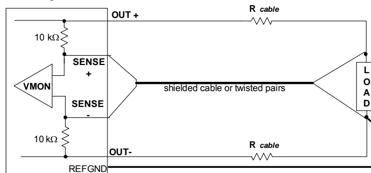
Fig. 4.2 - Remote voltage sensing scheme
