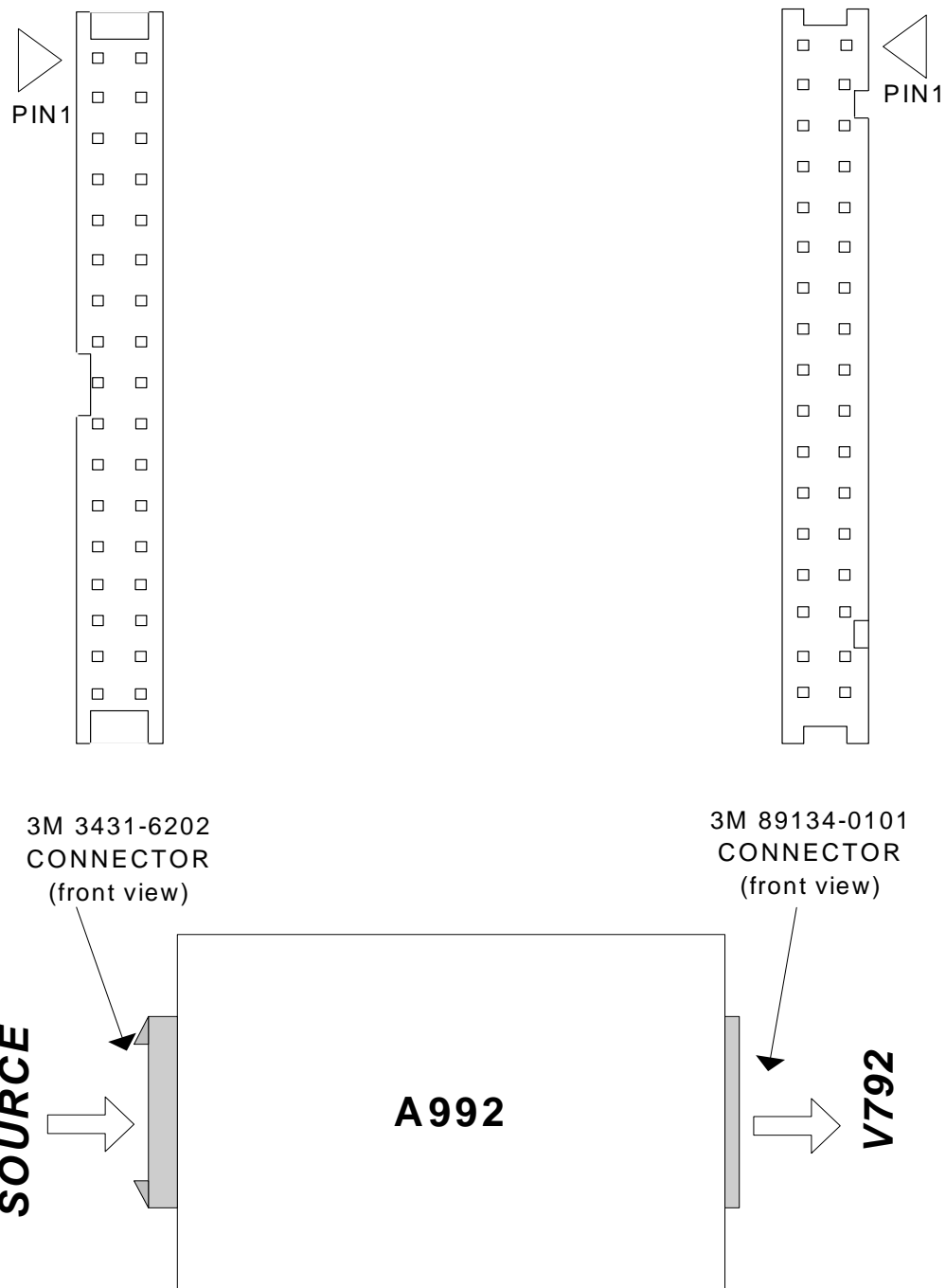
Fig. 2.1- The Mod. A992 input and output connectors
