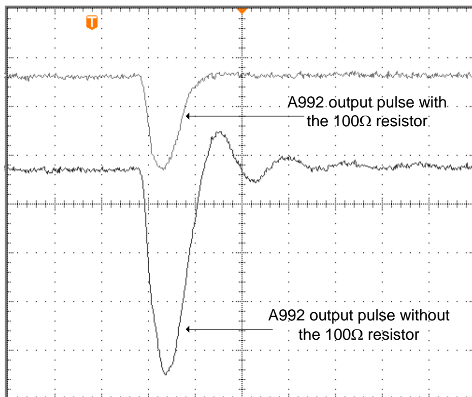
Fig. 3.2 – Effect of the 100 Ohm resistor on the A992 output pulses
