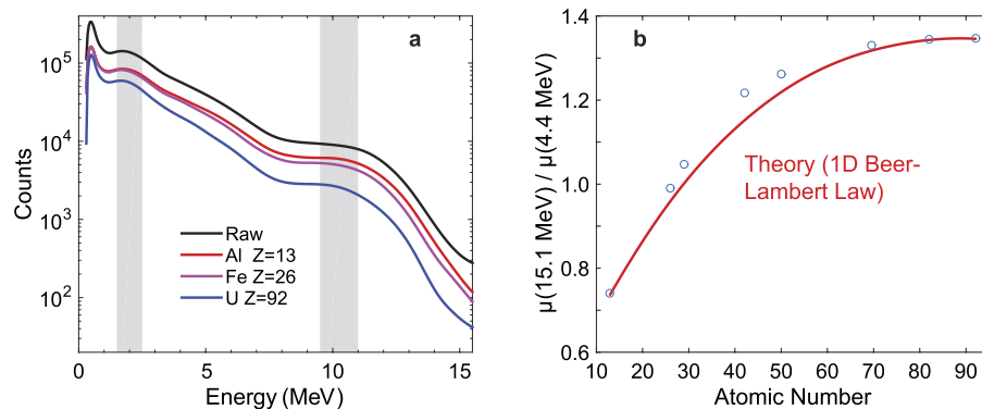
Figure 2. Response of Cherenkov detectors to various materials of the same aerial density. (a) Energy-dependent transmission measurement of several objects composed of different materials (a complete set of objects measured is provided in Supplementary Materials). The shaded regions of the spectrum are attributed to the Cherenkov detector response to 4.438 MeV and 15.1 MeV gamma rays produced in the ^{11}\text{B}(\text{d},\text{n})^{12}\text{C} reaction. (b) The two characteristic energy regions in (a) are used to reconstruct the effective atomic number of eight test objects composed of different materials. The known photon interaction cross sections for 4.438 MeV and 15.1 MeV gamma rays are used for a comparison calculation and shown as red line. The reconstruction method for the measured Cherenkov radiation spectrum and the comparison transmission calculation are described in detail in the Supplementary Materials. Error bars calculated for the measured ratios are smaller than the plot markers (circles) and are therefore not shown.
